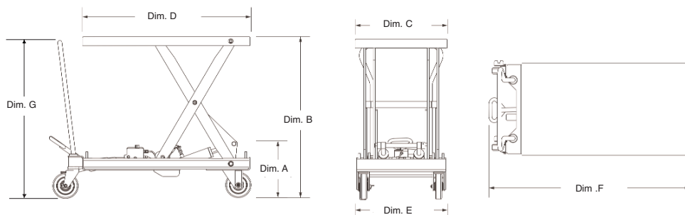
Selector Table for BX Series Mobile Lift Tables
